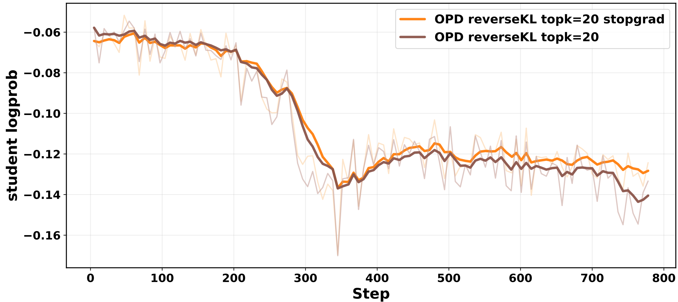
train/student_logprob
